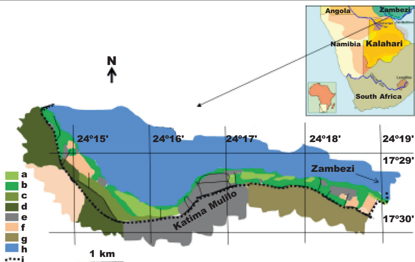
Fig. 1. Distribution of breeding pairs/occupied territories/cooperatives groups of the: kingfishers, bee-eaters, rollers, and hoopoes and woodhoopoes in a Zambezi Forest in NE Namibia: a, Zambezi riparian forest; b, grassland (flooded area); c, Colophospermum mopane forest; d, Kalahari woodland; e, arable grounds; f, urbanized built-up areas; g, rural area; h, Zambezi River; i, border of the study area.
